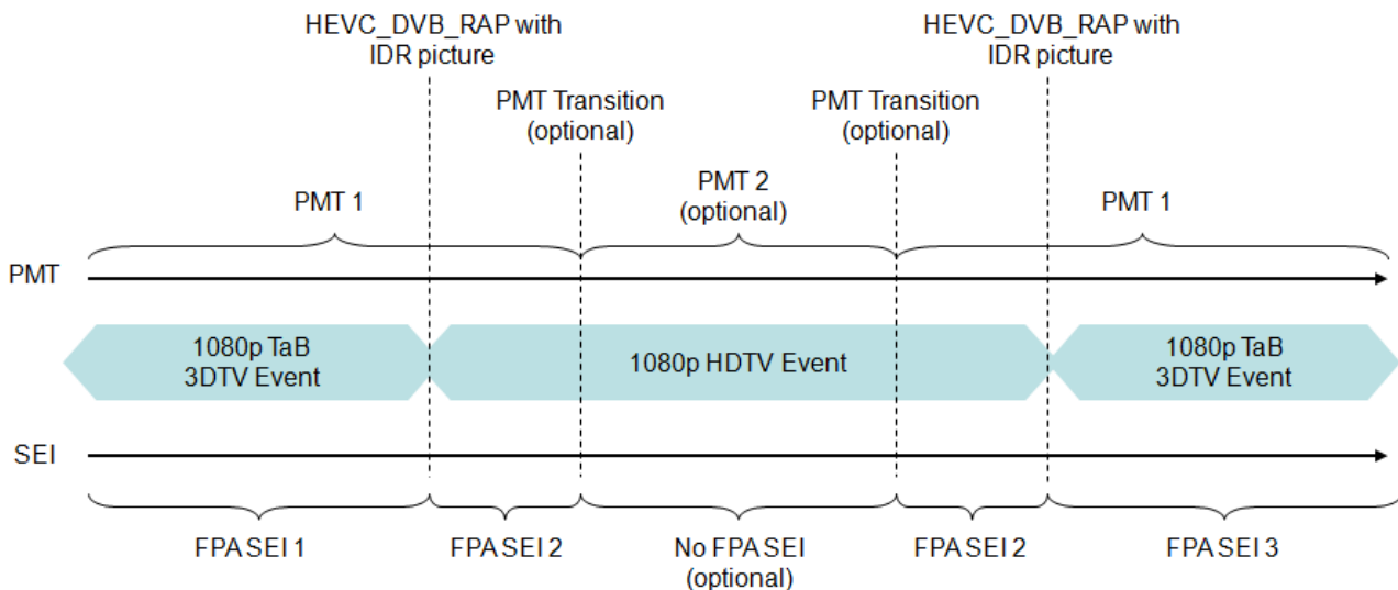
Figure 7: Generic scenarios of service frame compatible plano-stereoscopic 3DTV service format transitions
