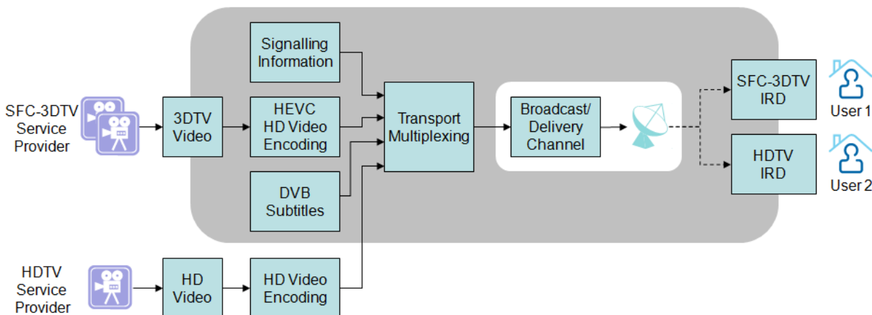
Figure 1: Scope of the service frame compatible plano-stereoscopic 3DTV specification
