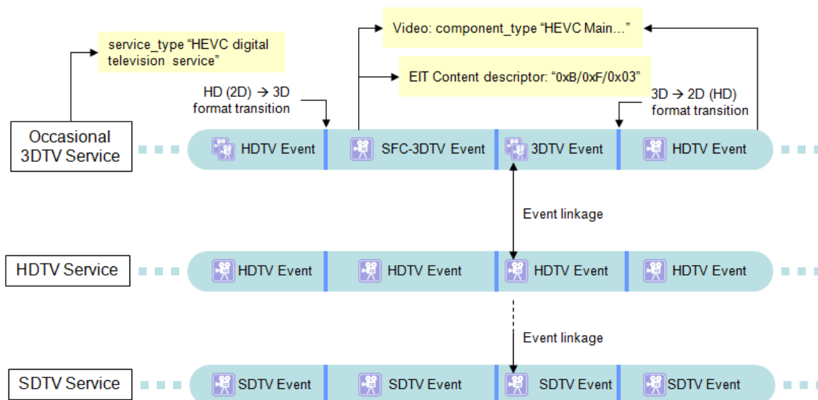
Figure 2: Service compatible frame compatible plano-stereoscopic 3DTV service scenarios
