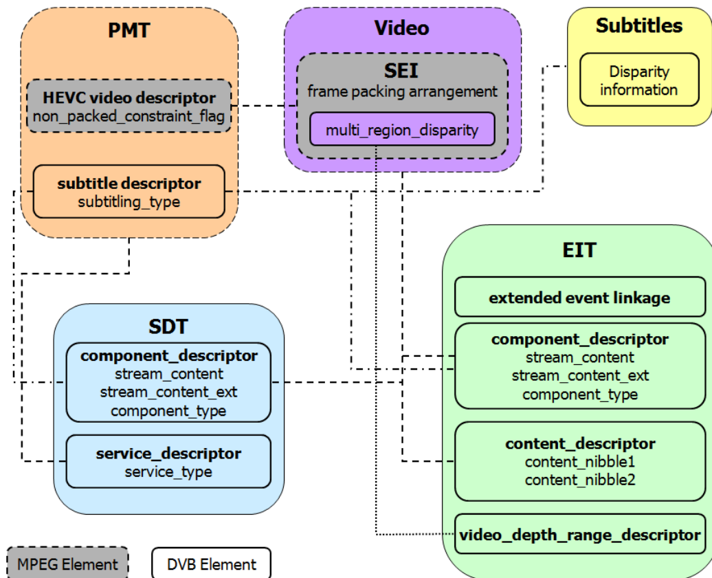
Figure 4: Elements of service frame compatible plano-stereoscopic 3DTV signalling
