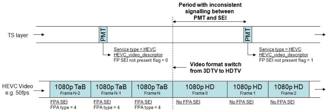
Figure 5: Example video format transition without transition assistance signalling
