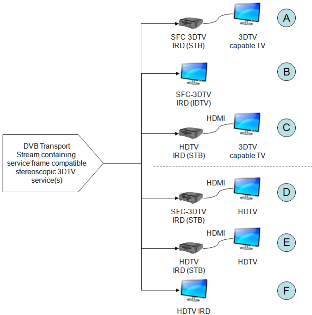
Figure 3: Service frame compatible plano-stereoscopic 3DTV IRD scenarios
