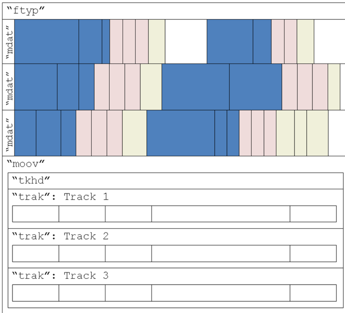
Figure 2: An example of basic file layout with "mdat" boxes preceding "moov" box
