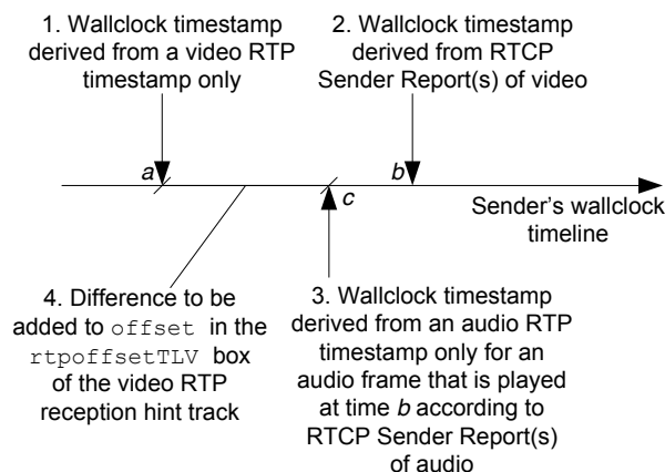
Figure 9. An example of correcting the lip synchronization in the RTP timestamp representation.
