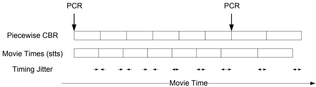
Figure 11: Timing jitter between PLCBR and values stored in “stts” box
