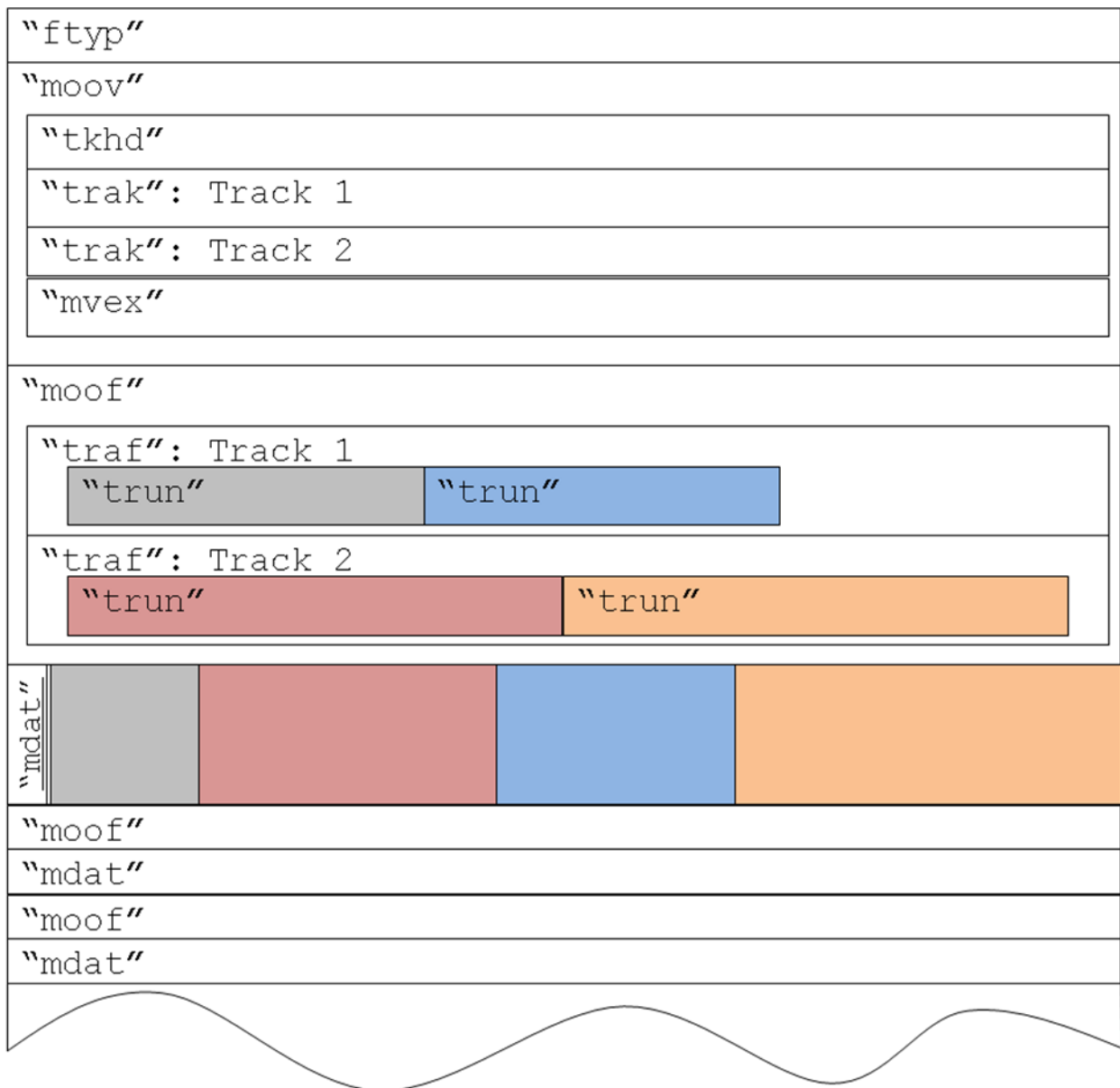
Figure 13: Example Layout of Fragmented File
