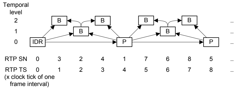
Figure 7. An example of a hierarchically temporally scalable bitstream with GOP_size equal to 4.
