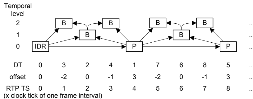
Figure 8. An example of setting the decoding time (DT) and the value of offset in the rtpoffsetTLV box of a hierarchically temporally scalable bitstream with GOP_size equal to 4.
