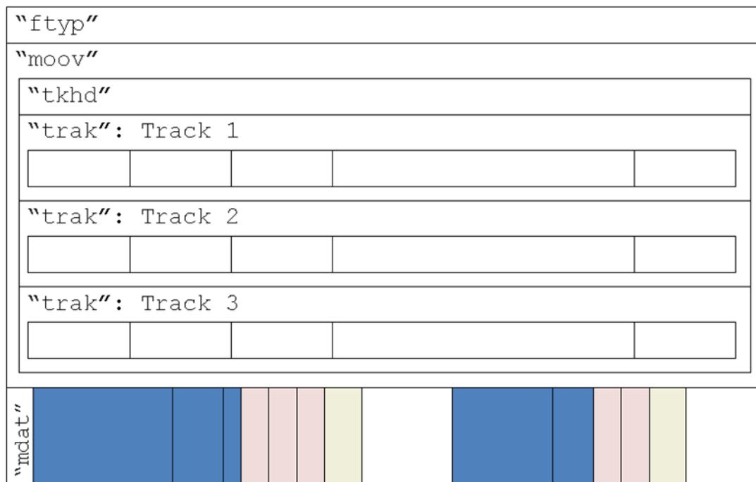
Figure 1: An example of basic file layout with “moov” box preceding single “mdat” box
