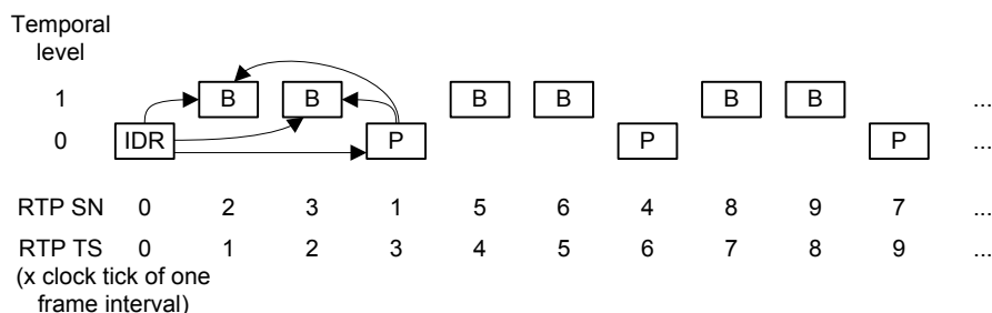
Figure 6. An example of a temporally scalable bitstream with GOP_size equal to 3.
