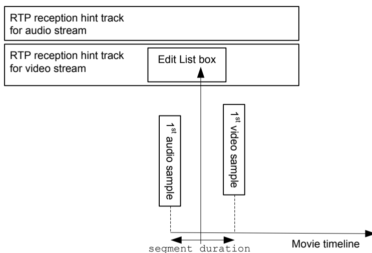
Figure 4. An example of creation of an Edit List box to compensate the unequal starting of the received RTP streams. segment_duration is copied to the first entry of the Edit List box.
