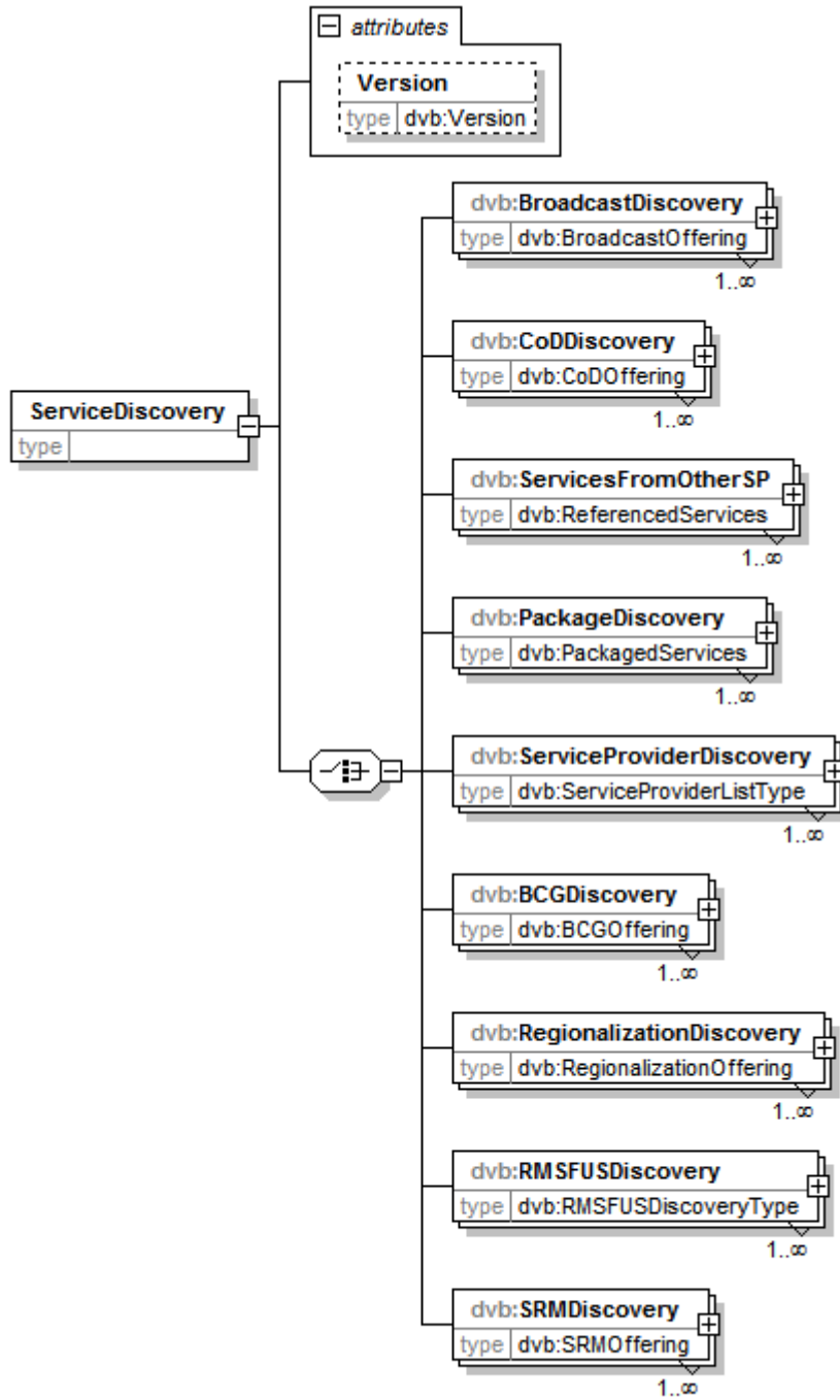
Figure C.332: Service discovery
