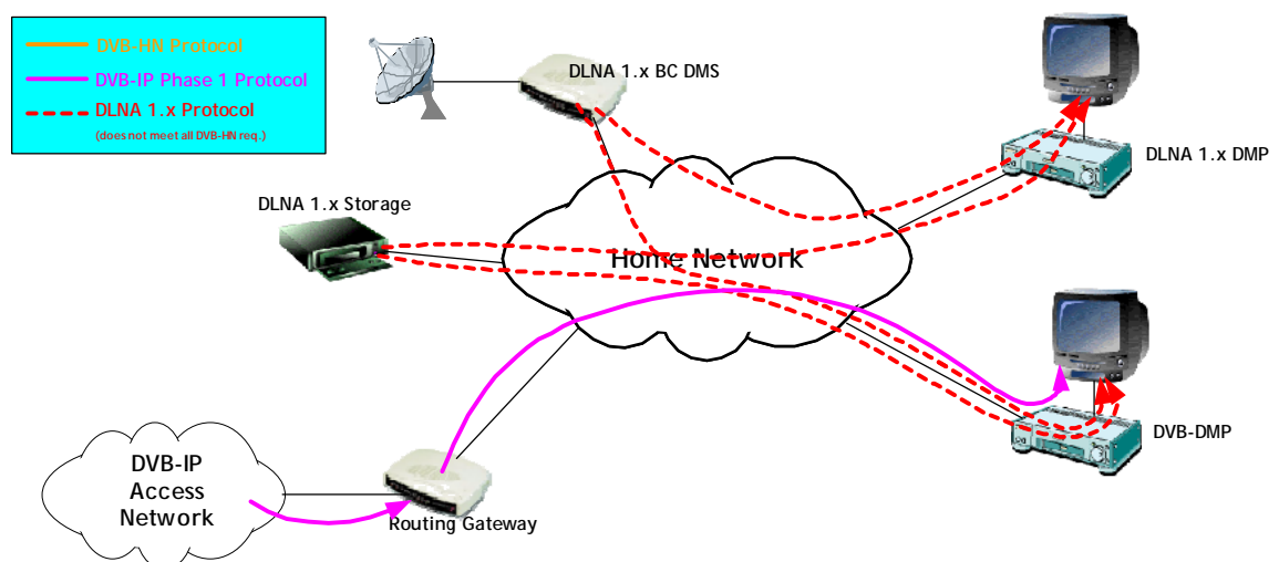
Figure 3.2: Home network consisting of DLNA devices and a DVB-HN DMR/P. The HN is connected to the DVB-IP access network via a routing gateway. DVB-IPTV services are played on the DVB-HN DMR/P.
