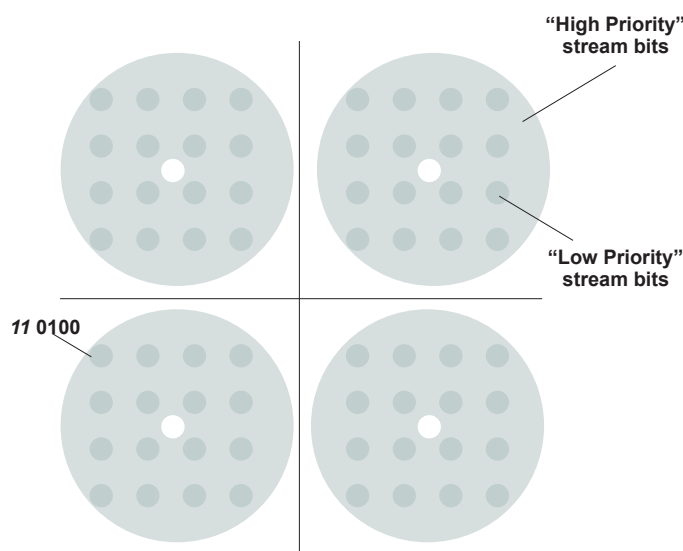
DVB-T Hierarchical 64QAM constellation with an embedded QPSK stream
