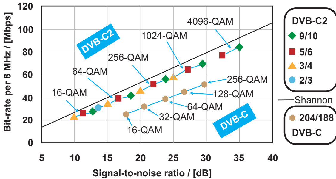
Figure 2. DVB-C2 noise performance compared to DVB-C
